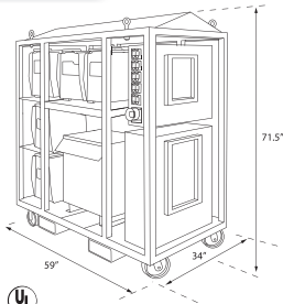
Power Panel
